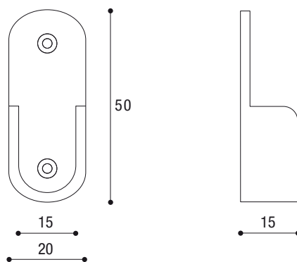
Reggitubo ovale Oval tube support
