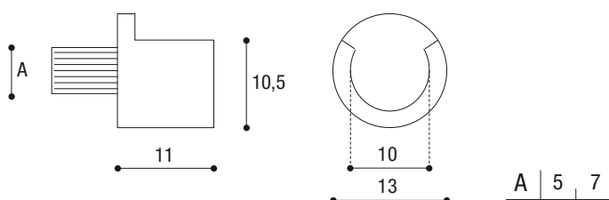
Reggitubo per scarpiera Tube support for shoe rack
