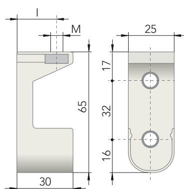
Reggitubo ovale Oval tube support
