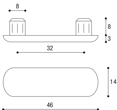
Pattino a due perni Slider with two pins
