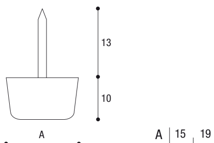
Piedino sottosedia Pratic alto High Pratic bearing
