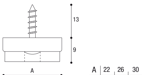
Piedino sottosedia con feltro a vite Felt bearing with screw
