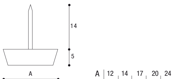
Piedino sottosedia Pratic Pratic bearing
