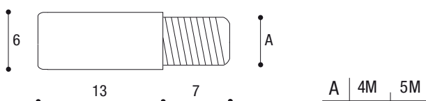
Perno filettato per reggicristalli piani e a ventosa Threaded pin for shelf support for glass with plane and suction cap
