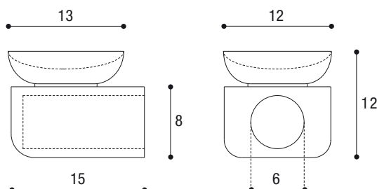
Reggicristallo a ventosa Shelf support for glass with suction cap
