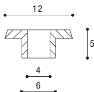
Reggicristallo piano Flat shelf support for glass
