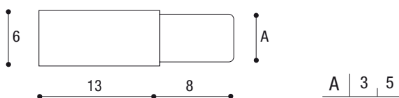
Perno per reggicristalli piani e a ventosa Pin for shelf support for glass with plane and suction cap
